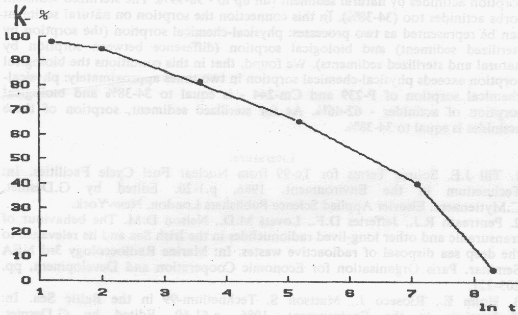
Figure 1. Kinetic of technetium-99 sorption by natural sediment from lake water at solid/liquid ratio = 2.3 \cdot 10^{-2} g/ml. K - specific radioactivity of solution, % t - time, hours
