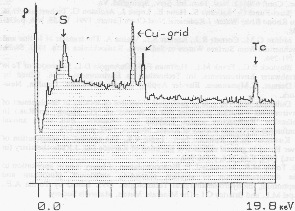
Figure 2. Elemental X-ray microanalysis of sediment, which was formed by sulfatereducing bacteria in nutrient medium with 40 mg Tc/l.
